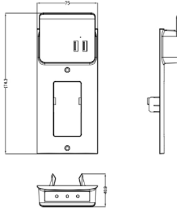
EPD-3128 Spec Dimensions: mm
