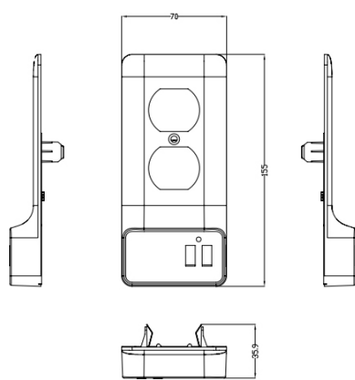
EPD-3028 Spec Dimensions: mm
